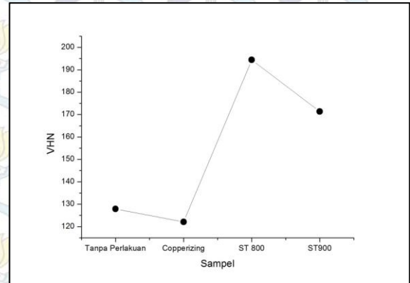
Gambar 8. Nilai Kekerasan Baja AISI 1006, Copperized -AISI 1006, dan Sampel Solution treatment .
