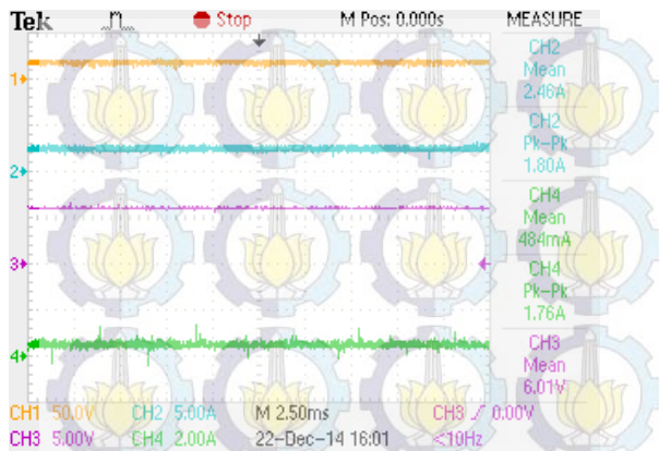
Gambar 14. Hasil pengujian prototype rangkaian Interleaved Boost Converter
