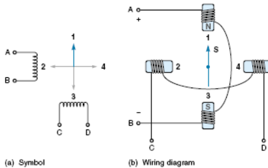
Gambar 2.7 Motor stepper dua-phase ( bipolar )
