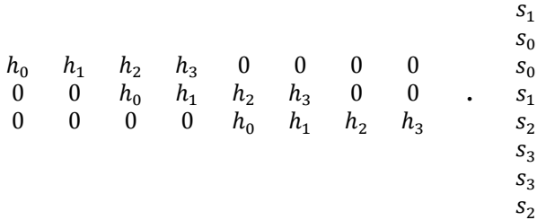
Gambar 2.4 Ilustrasi Low Pass Filter
