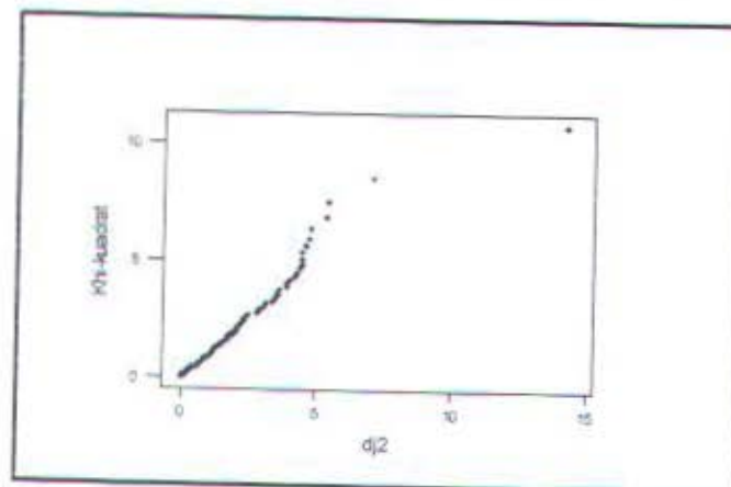
Gambar 4.4.1 Plot Multivariate Normal Residual
