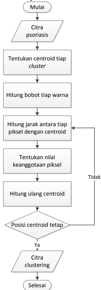
Gambar 3.3 Diagram alur W-k-means clustering
