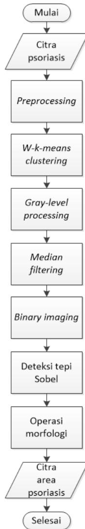
Gambar 3.1 Diagram alur sistem
