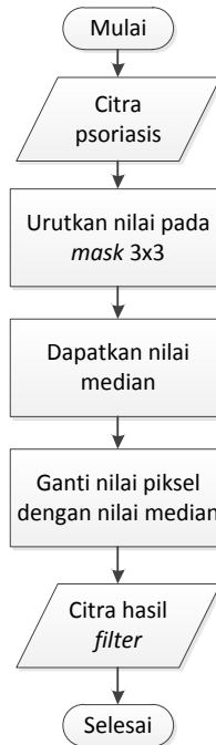
Gambar 3.4 Digram alur median filtering
