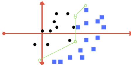
Gambar 2.2 Contoh Hyperplane
