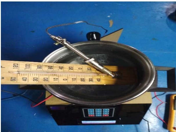
Gambar 4.1 Kalibrasi Termokopel
