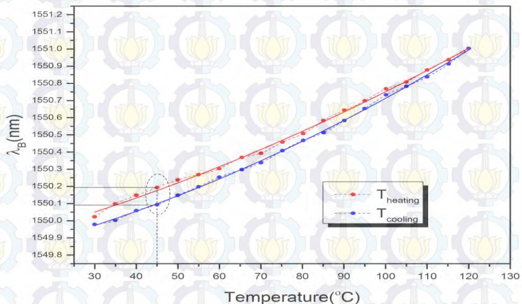
Gambar 4. 8. Hasil Uji Hysteresis Bare FBG
