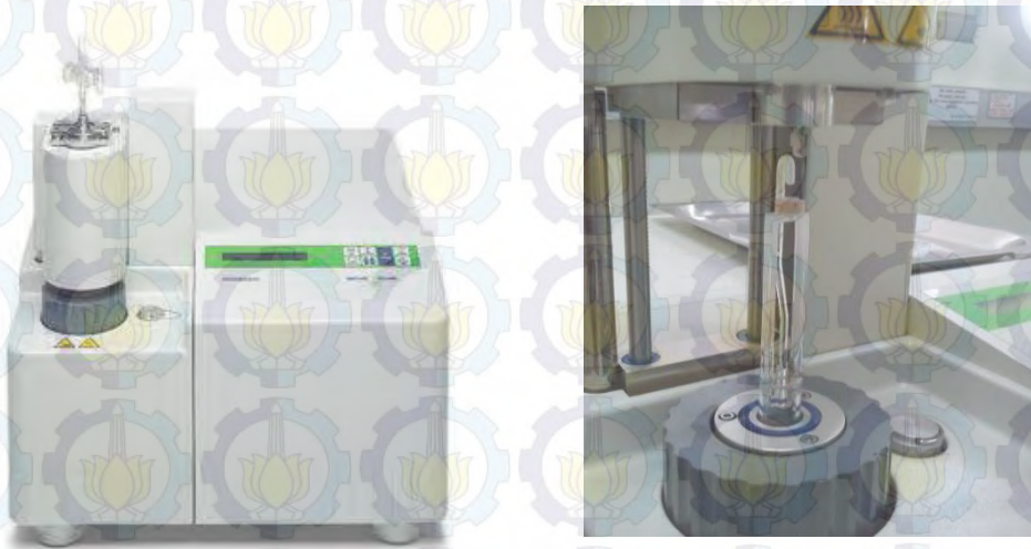
Gambar 4. 11.(a) Mettler Thermomechanical Analyser (TMASDTA840)-1 di Lab. Energi ITS, (b) Proses Pengukuran Koefisien Ekspansi Thermal Keramik Geopolimer
