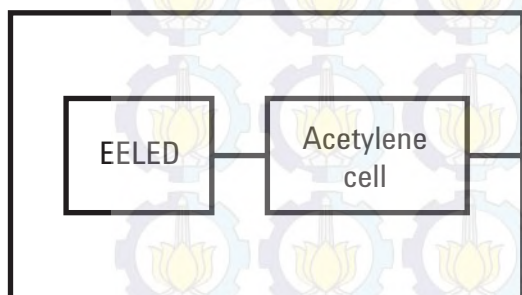
Figure 1. Wavelength calibrator block diagram
