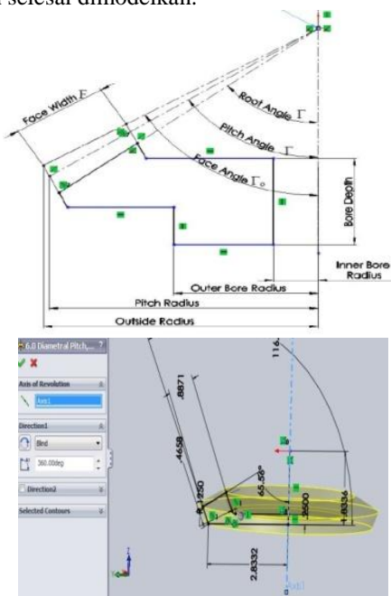
Gambar 4 Sket base bevel gear
