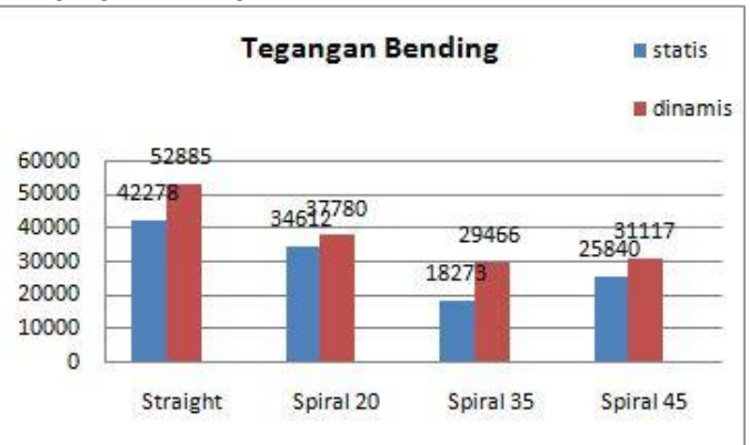
Gambar 9. Nilai Tegangan Bending
