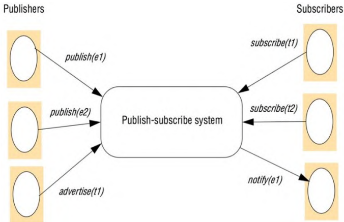
Gambar 2.1 Skema publish-subscribe
