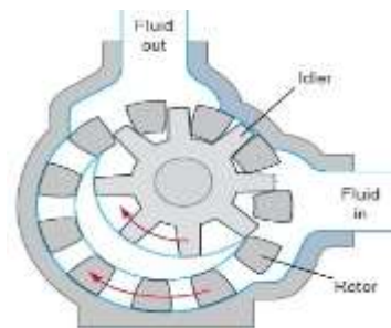
Gambar 3.8 Blower positive displacement
