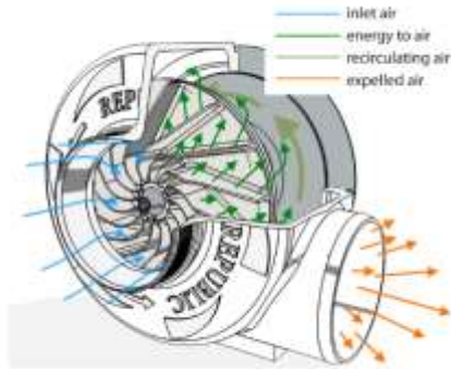
Gambar 3.7 Blower Sentrifugal
