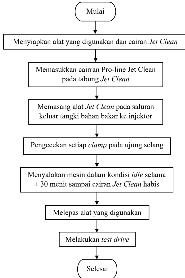
Gambar 5. 4 Diagram Alir Proses Jet Clean
